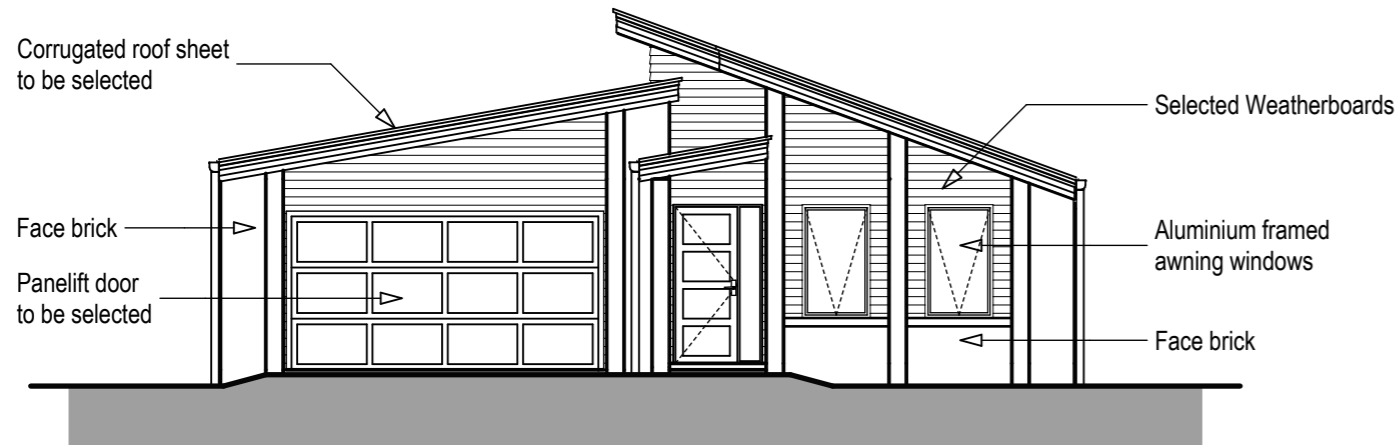
Elevation - Option 1
